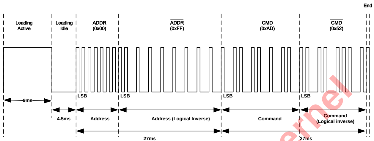
Fig VII.42.3. Data Frame
