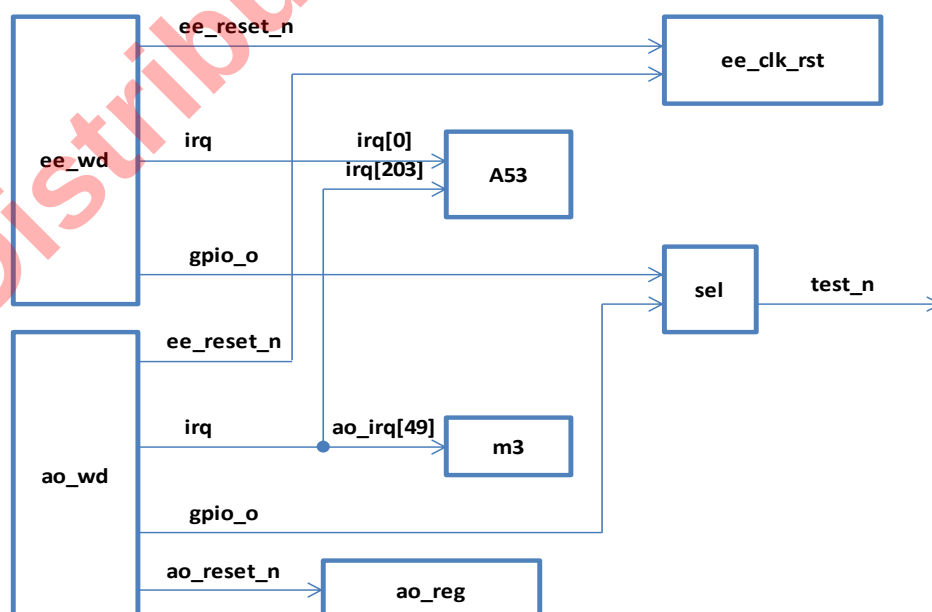
Figure 26.1 Watchdog Timer
