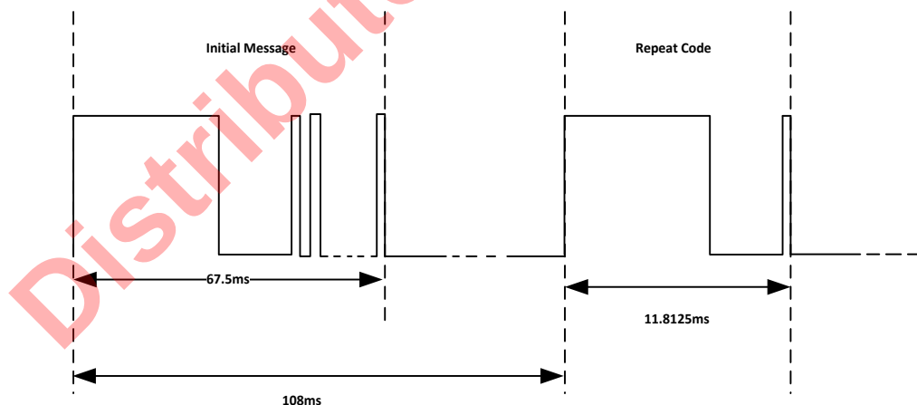
Fig VII.42.4. Repeat Code
