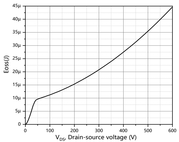
Figure 10. Typ. Coss stored energy
