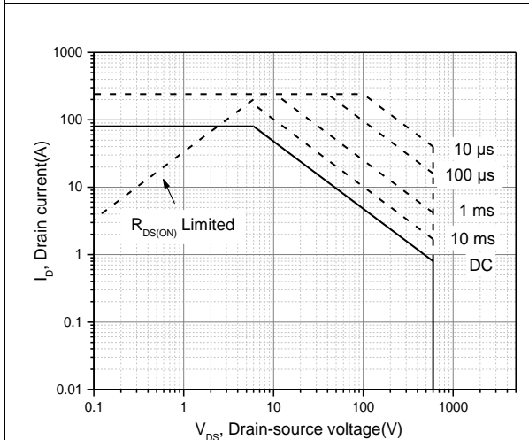
Figure 11. Safe operation area T_C=25\text{ °C}
