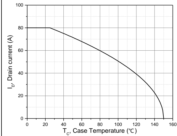
Figure 9. Drain current
