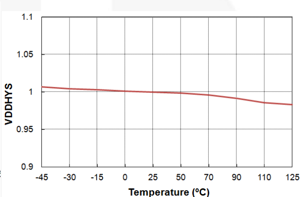
Figure 19. VDDHYS vs. Temperature
