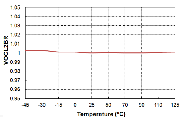
Figure 47. VOCL2BR vs. Temperature
