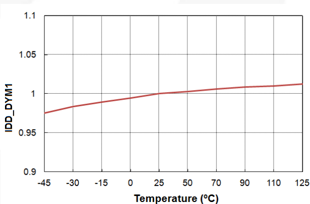
Figure 15. IDD_DYM1 vs. Temperature
