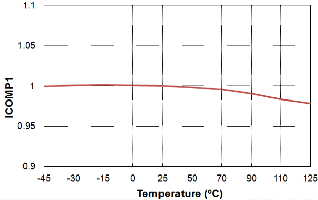
Figure 21. ICOMP1 vs. Temperature
