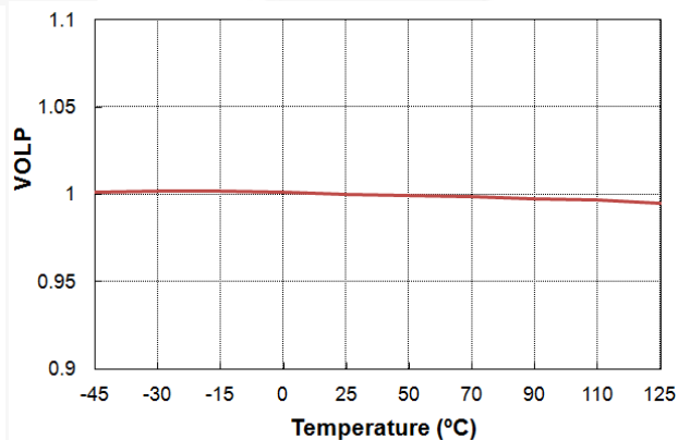
Figure 31. VOLP vs. Temperature
