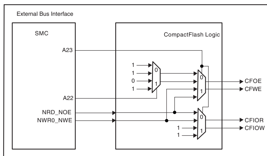
Figure 19-4. CompactFlash Read/Write Control Signals
